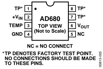
Figure 3. 8-Lead PDIP and SOIC Pin Configuration
