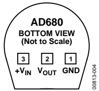
Figure 4. Connection Diagram
