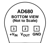
Figure 2. Connection Diagram
